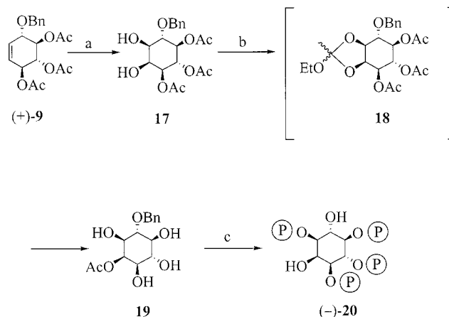
Scheme 6. Reagents and conditions: (a) RuCl 3 , NaIO 4 , acetonitrile. (b) 1. MeC(OEt) 3 , p -TSA; 2. NaOMe, MeOH; 3. 80% HOAc (99%). (c) 1. (1,5-Dihydro-2,4,3-benzodioxaphosphhepin-3-yl)diethylamine, 1 H -tetrazole, CH 2 Cl 2 , then m -CPBA; 2. Pd/C, H 2 , ethanol/water; 3. 0.25 N NaOH (over all steps 20%).
