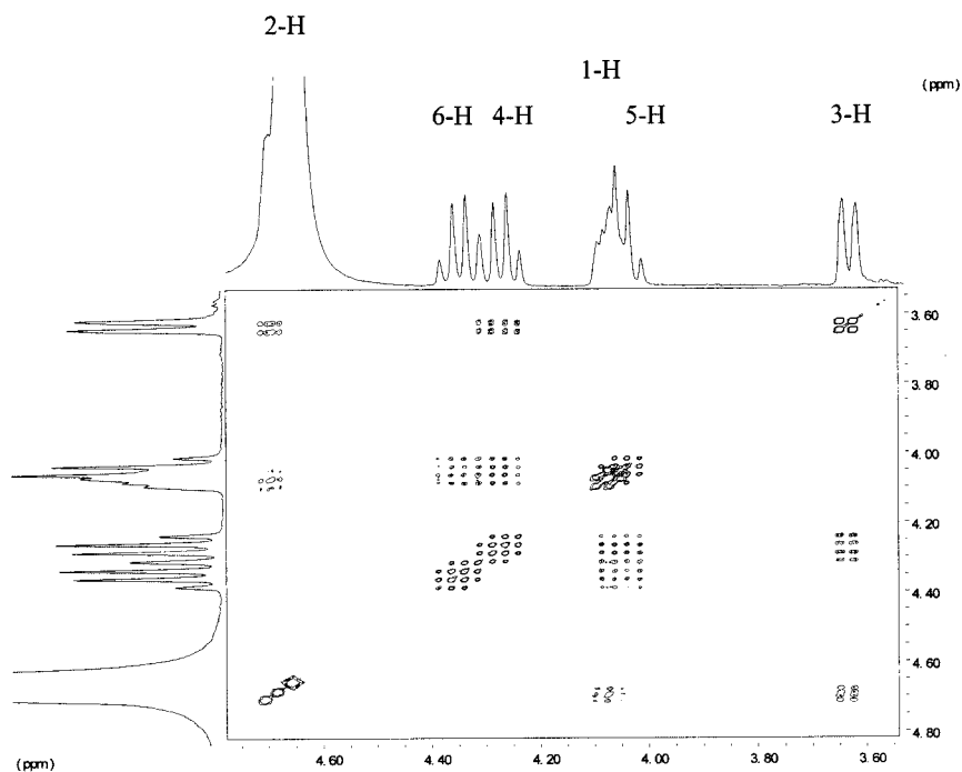
Figure 2. ^1\text{H} - ^1\text{H} COSY spectrum of myo -Ins(1,2,4,5,6) \text{P}_5 [–]- 16 .
