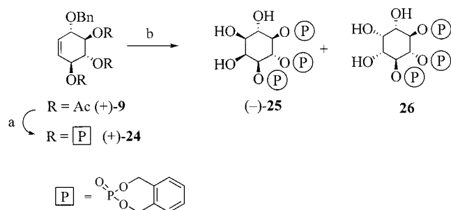
Scheme 8. Reagents and conditions: (a) 1. NaOMe, MeOH; 2. (1,5-dihydro-2,4,3-benzodioxaphosphepin-3-yl)diethylamine, 1 H -tetrazole, CH 2 Cl 2 , then m -CPBA. (b) 1. RuCl 3 , NaIO 4 , acetonitrile; 2. Pd/C, H 2 , ethanol/water.
