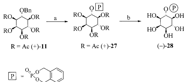
Scheme 9. Reagents and conditions: (a) 1. Pd/C, H 2 , EtOAc (99%); 2. (1,5-dihydro-2,4,3-benzodioxaphosphepin-3-yl)diethylamine, 1 H -tetrazole, CH 2 Cl 2 , then m -CPBA (51%). (b) 1. Pd/C, H 2 , ethanol/water; 2. 0.25 N NaOH (99%).
