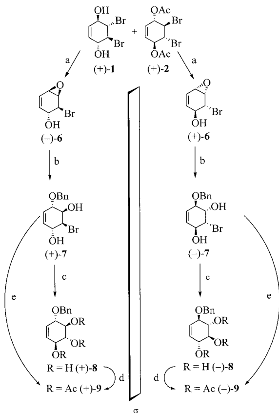
Scheme 2. Reagents and conditions: (a) LiOH, Et 2 O/MeOH (92%). (b) BnOH, CH 2 Cl 2 , H 2 SO 4 (cat.) (99%). (c) 1. LiOH, Et 2 O/MeOH (99%); 2. p -TSA, H 2 O (after crystallization <30%). (d) Ac 2 O, pyridine (99%). (e) 1. Ac 2 O, pyridine (100%); 2. KOAc, glacial AcOH/Ac 2 O, 5 d, 125 °C (55%).
