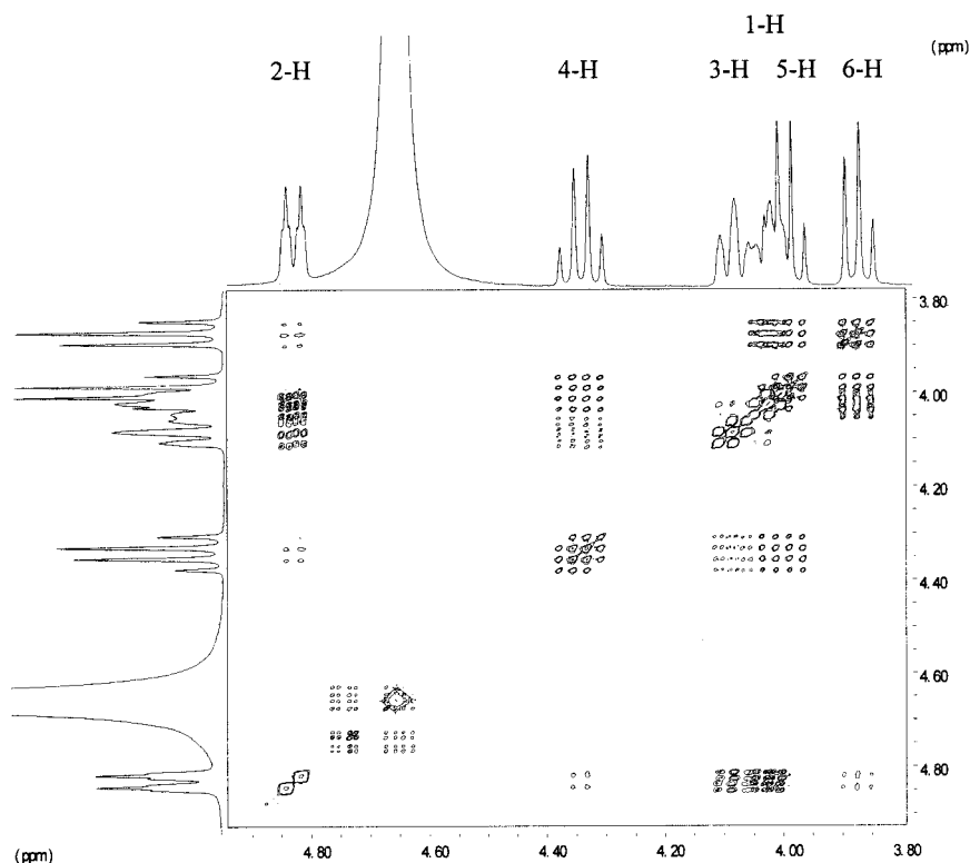
Figure 1. ^1\text{H} - ^1\text{H} COSY spectrum of myo -Ins(1,2,3,4,5) \text{P}_5 (–)- 15 .
