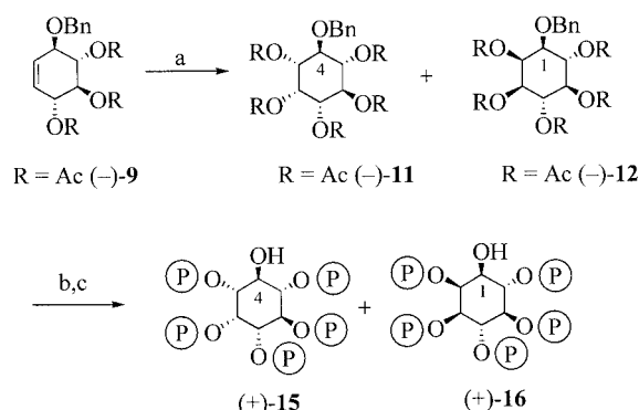
Scheme 5. Reagents and conditions: (a) 1. \text{RuCl}_3 , \text{NaIO}_4 , acetonitrile; 2. \text{Ac}_2\text{O} , pyridine (99%). (b) NaOMe, MeOH (99%). (c) 1. (1,5-Dihydro-2,4,3-benzodioxaphosphepin-3-yl)diethylamine, 1 H -tetrazole, \text{CH}_2\text{Cl}_2 , then m -CPBA (50%); 2. Pd/C, \text{H}_2 , ethanol/water (99%).
