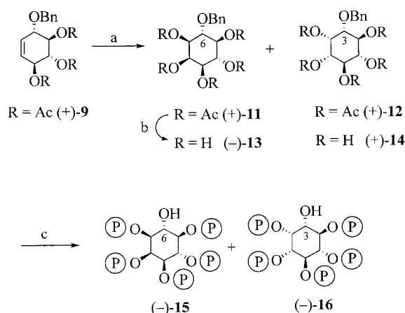
Scheme 4. Reagents and conditions: (a) 1. \text{RuCl}_3 , \text{NaIO}_4 , acetonitrile; 2. \text{Ac}_2\text{O} , pyridine (99%). (b) NaOMe, MeOH (99%). (c) 1. (1,5-Dihydro-2,4,3-benzodioxaphosphepin-3-yl)diethylamine, 1 H -tetrazole, \text{CH}_2\text{Cl}_2 , then m -CPBA (50%); 2. Pd/C, \text{H}_2 , ethanol/water (99%).
