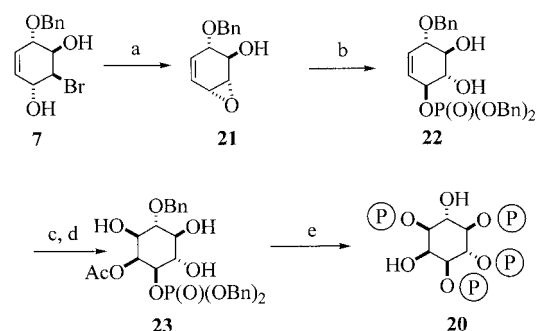
Scheme 7. Reagents and conditions: (a) LiOH, Et 2 O/MeOH. (b) CH 2 Cl 2 , dibenzyl phosphate (40%). (c) RuCl 3 , NaIO 4 , CH 2 Cl 2 , acetonitrile. (99%). (d) 1. MeC(OEt) 3 , p -TSA; 2. 80% HOAc (92%). (e) 1. (1,5-Dihydro-2,4,3-benzodioxaphosphhepin-3-yl)diethylamine, 1 H -tetrazole, CH 2 Cl 2 , then m -CPBA; 2. Pd/C, H 2 , ethanol/water; 3. 0.25 N NaOH (40%).
