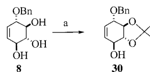
Scheme 10. Reagents and conditions: (a) 2,2-dimethoxypropane, anhydrous acetone, PPTSA, 3 d (80%).
